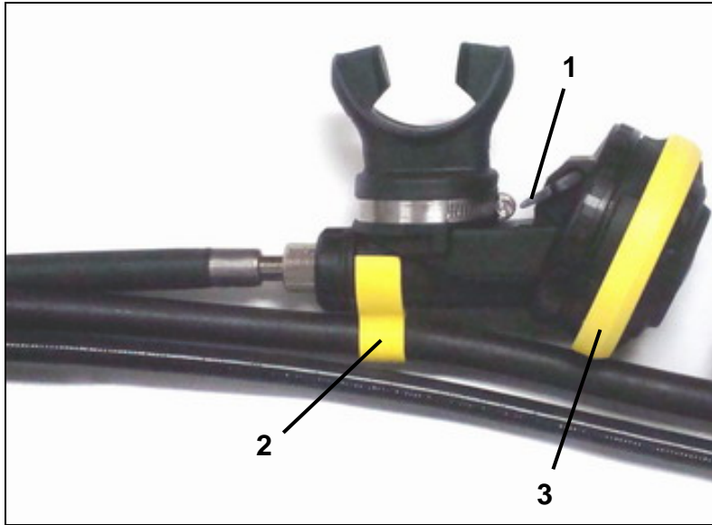
Overview of the Octopus Breathing Valve ( 1 - Locking Lever, 2 - Quick Snap Octopus Holder, 3 - Shield Ring)
